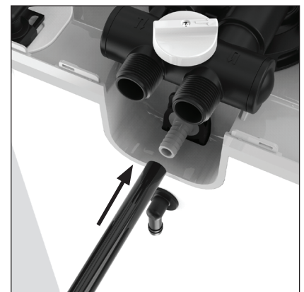
Figure 6: Connect Drain Line
